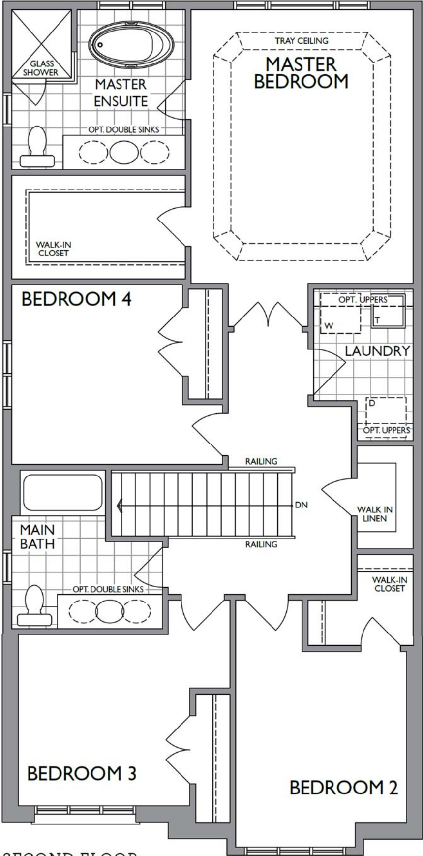
SECOND FLOOR ELEVATION E
