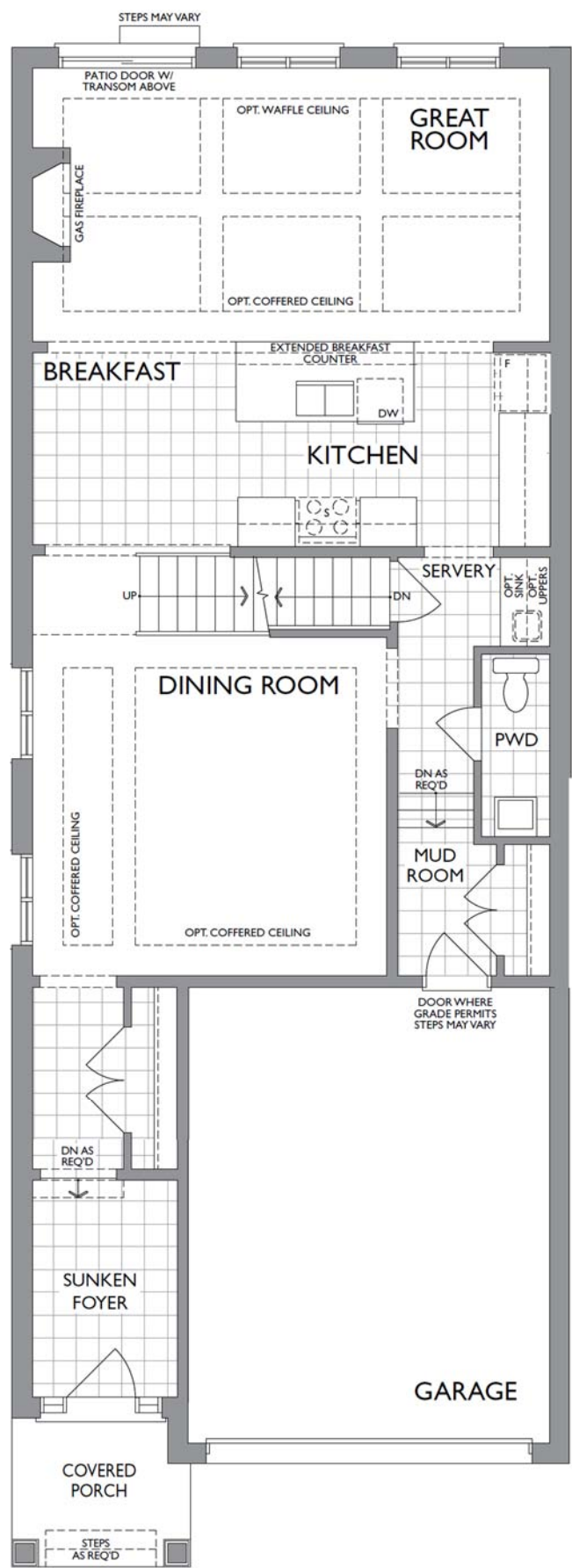
MAIN FLOOR ELEVATION D
