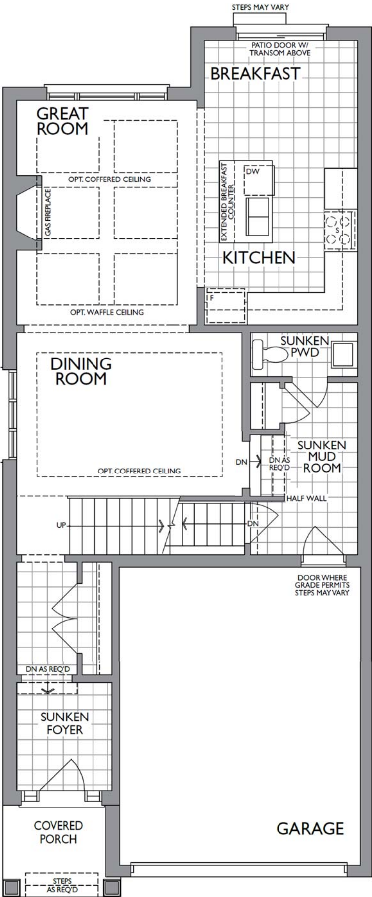
MAIN FLOOR ELEVATION C
