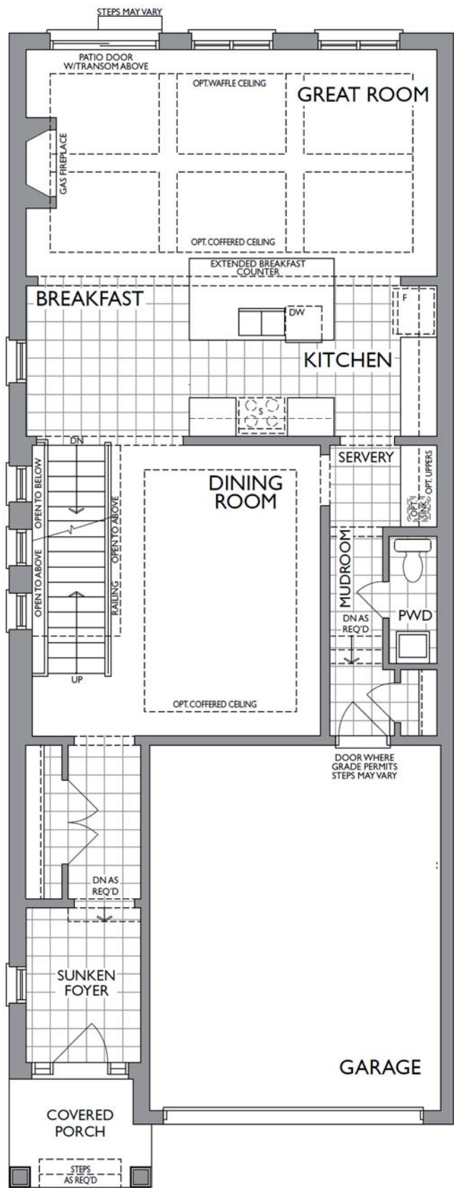
MAIN FLOOR ELEVATION C
