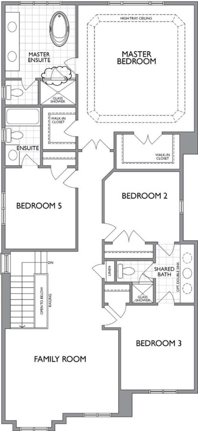
OPT. SECOND FLOOR WITH 4 BEDROOM & FAMILY ROOM ELEVATION A
