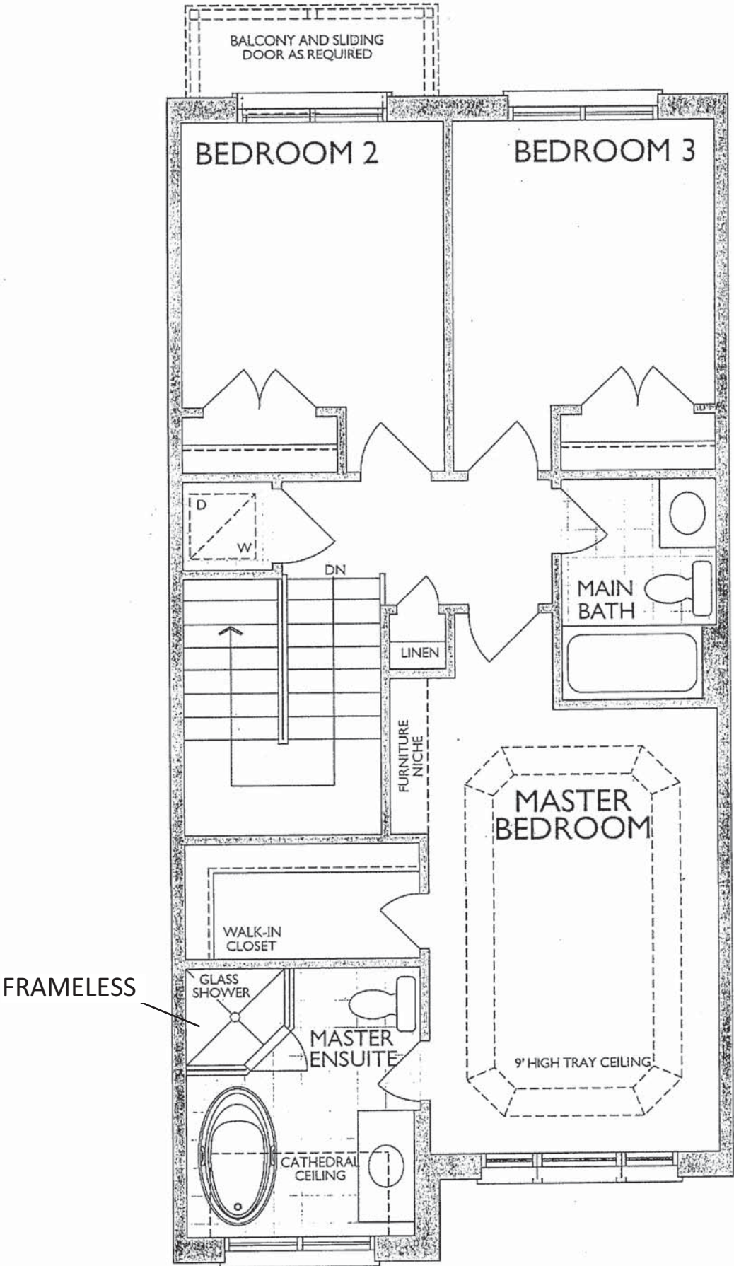
UPPER LEVEL ELEVATION B
