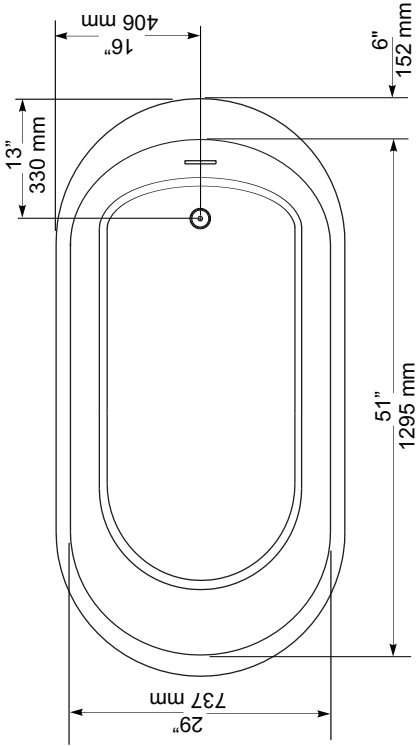
TOP VIEW
