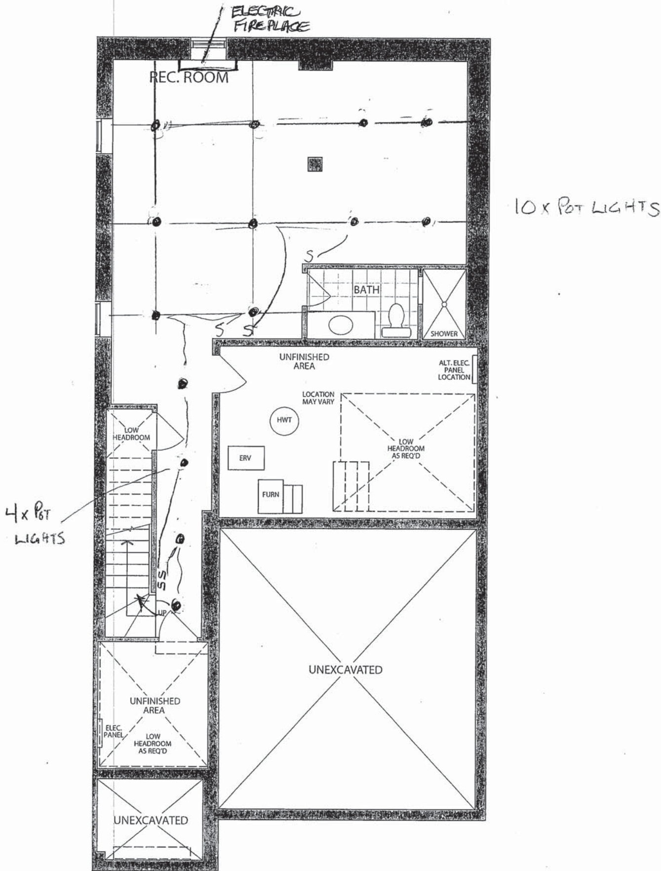
OPTIONAL FINISHED LOWER LEVEL ELEVATION A (ELEV. B & C SIMILAR)
