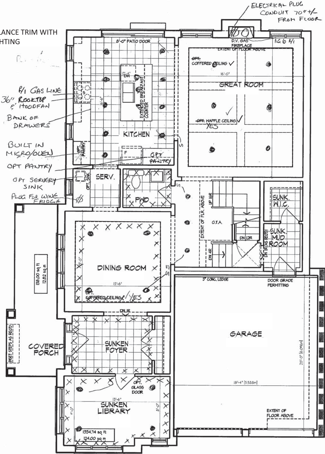
MAIN LEVEL ELEVATION A
