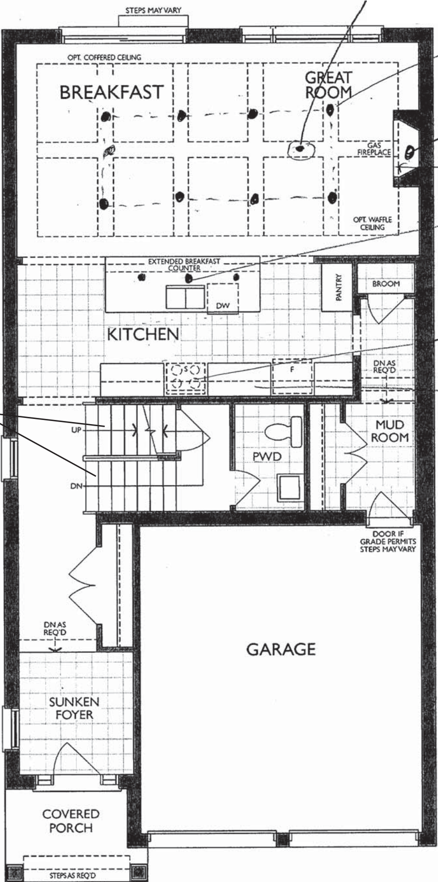
MAIN FLOOR ELEVATION B & C
