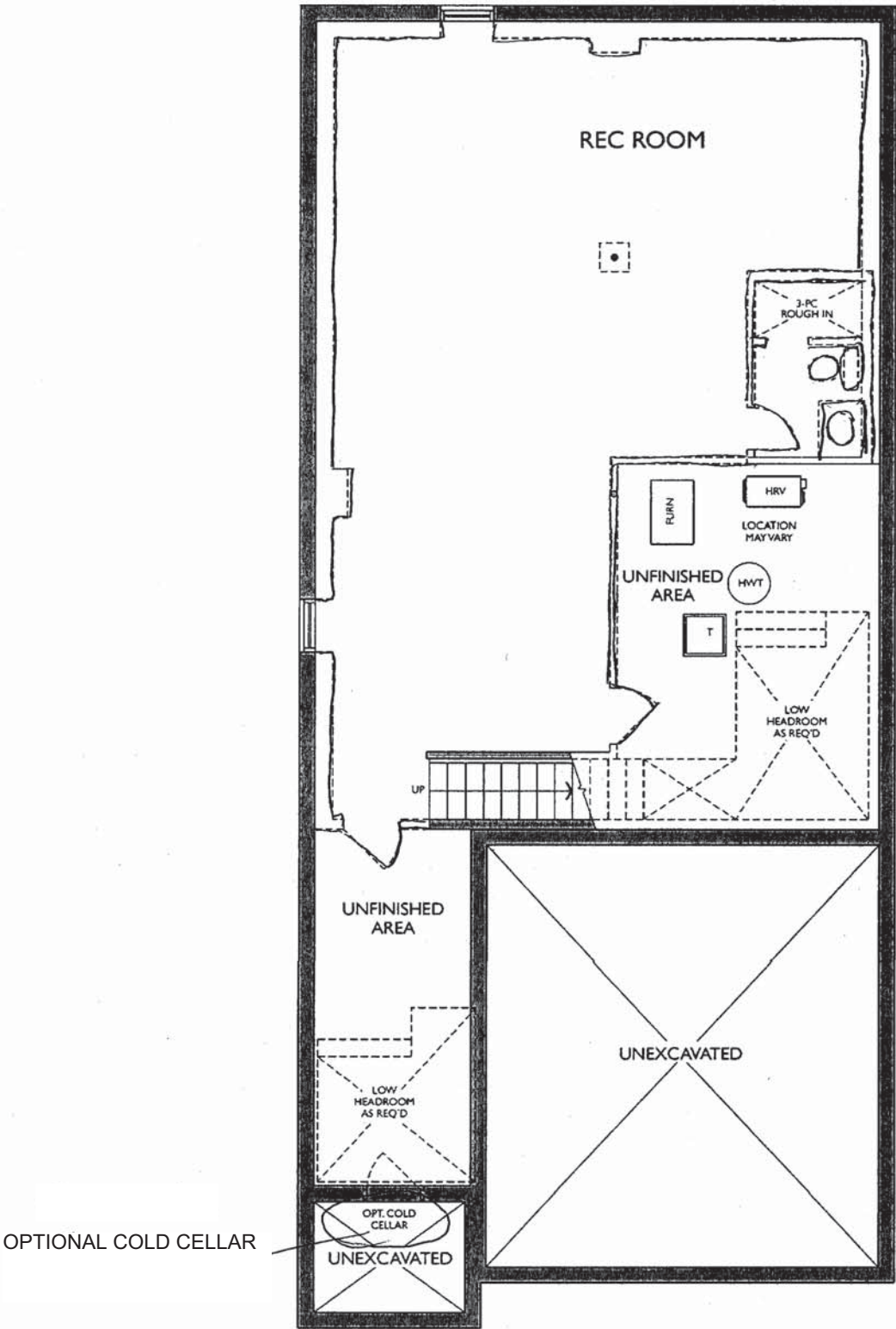
LOWER LEVEL ELEVATION C
