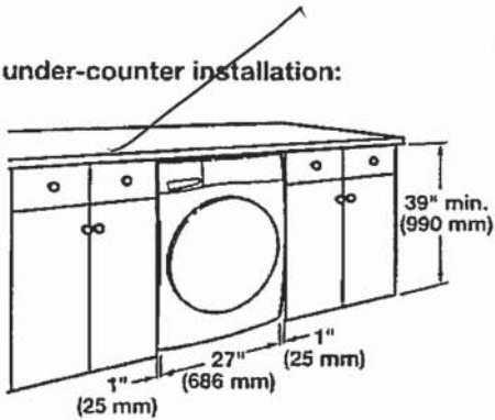
Recessed area or closet installation:
