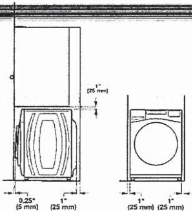
Custom cabinet installation:
