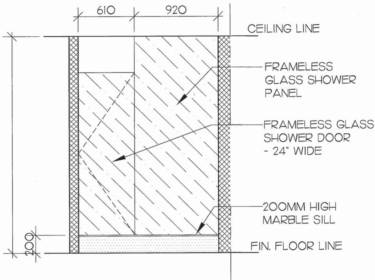
PART.ELEV. : SHOWER STALL
