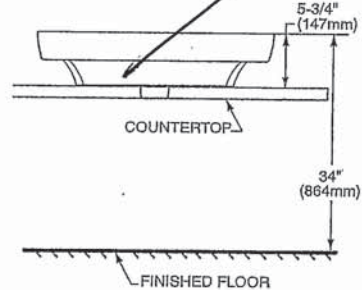
ABOVE COUNTER CONFIGURATION
