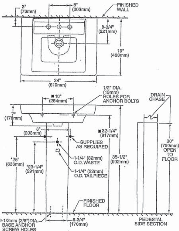
PEDESTAL CONFIGURATION (NOT ADA COMPLIANT)
