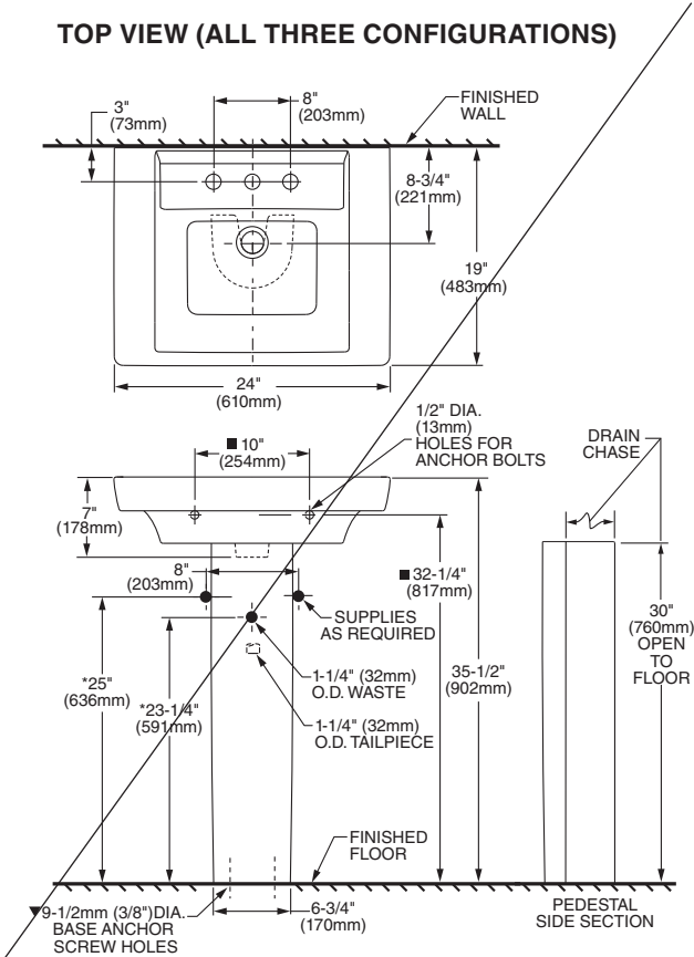
PEDESTAL CONFIGURATION (NOT ADA COMPLIANT)
