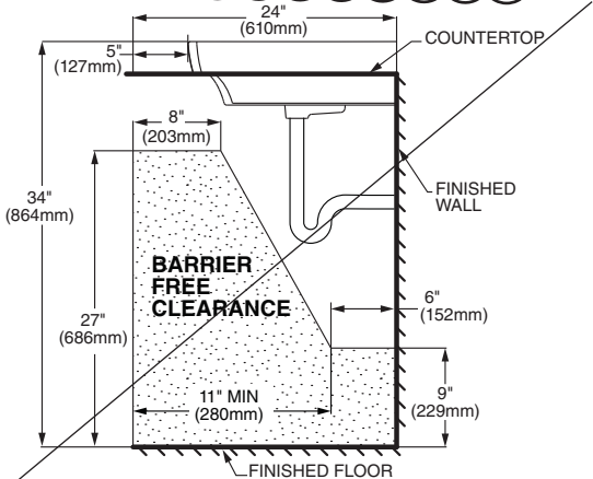
DROP-IN SINK CONFIGURATION
