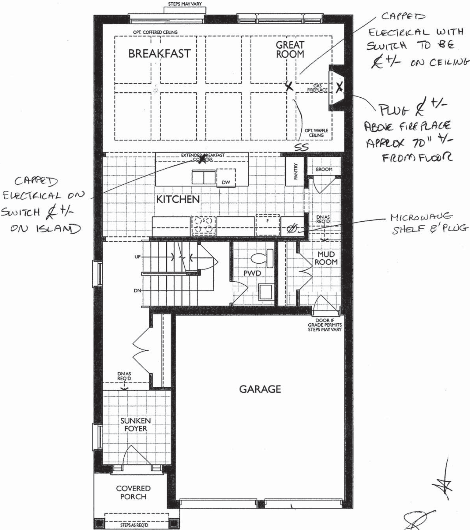
MAIN FLOOR ELEVATION B & C
