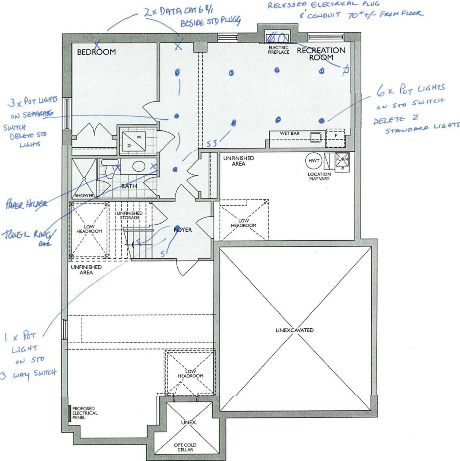
SPACES FINISHED LOWER LEVEL VERSION 2 ELEV. B
