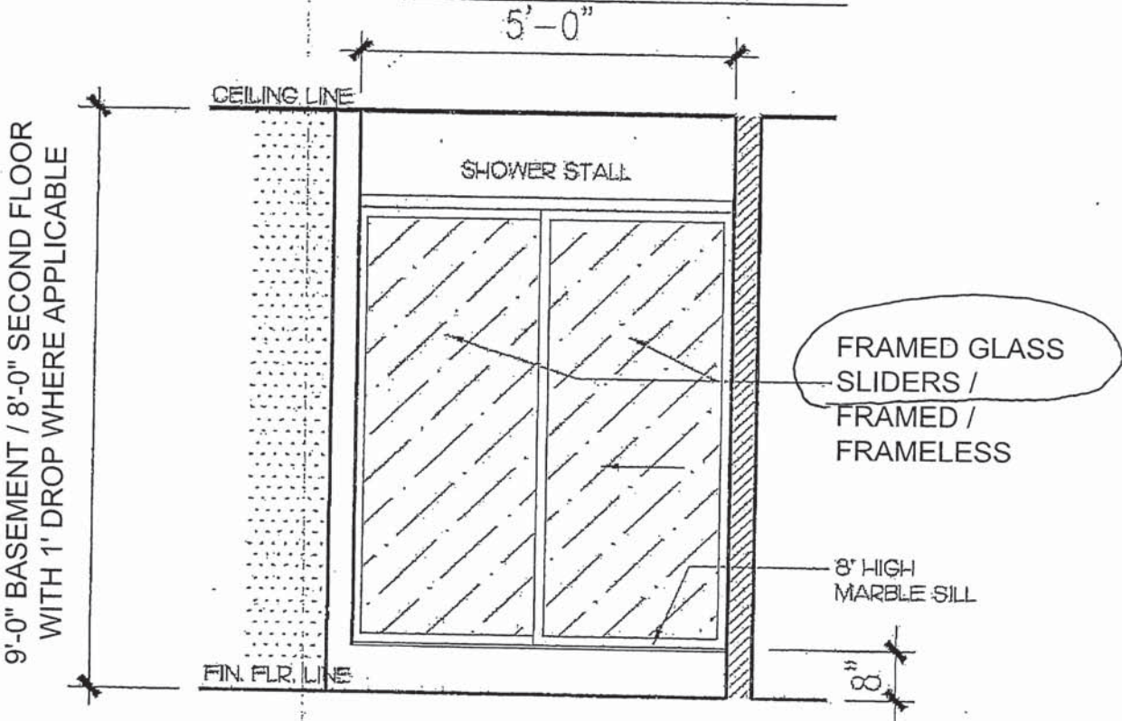
PART.ELEV. : SHOWER STALL
