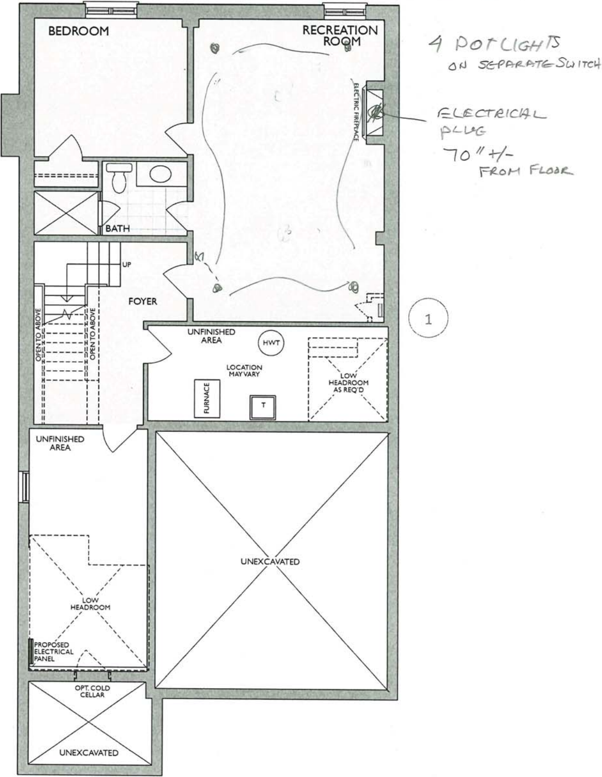
FINISHED LOWER LEVEL ELEV. A & B
