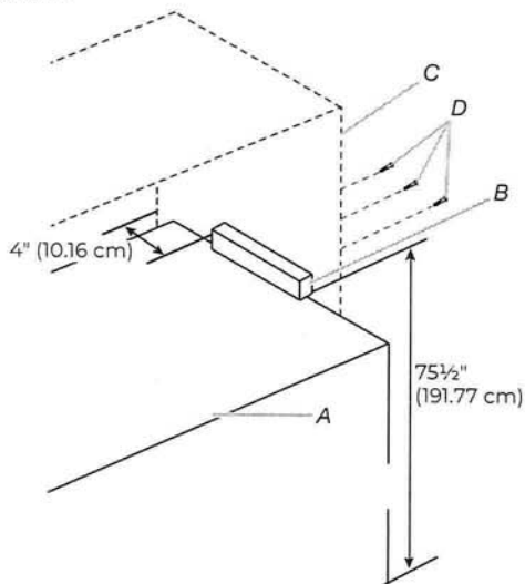
A. Refrigerator B. Secondary anti-tip board C. Kitchen cabinet D. Wood screws
