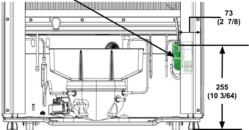
Water valve
