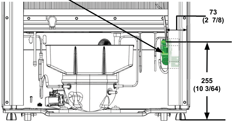
Water valve
