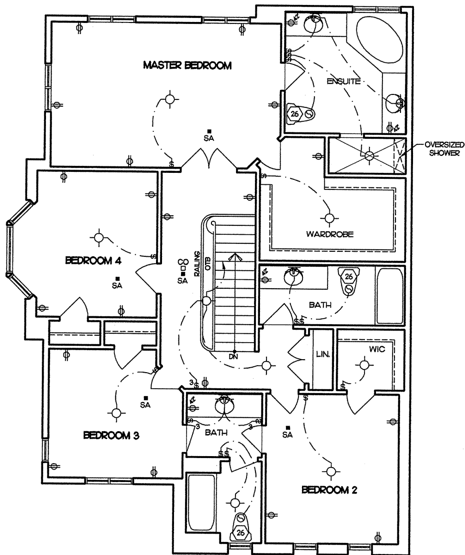
OPT. SECOND FLOOR PLAN
