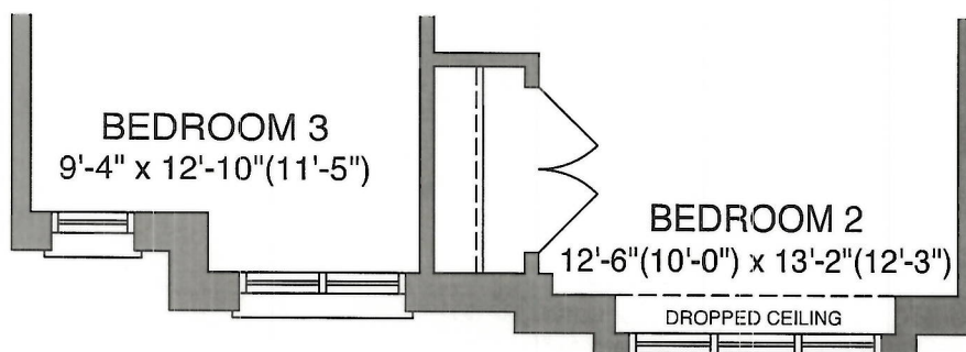
SECOND FLOOR - ELEV B2
