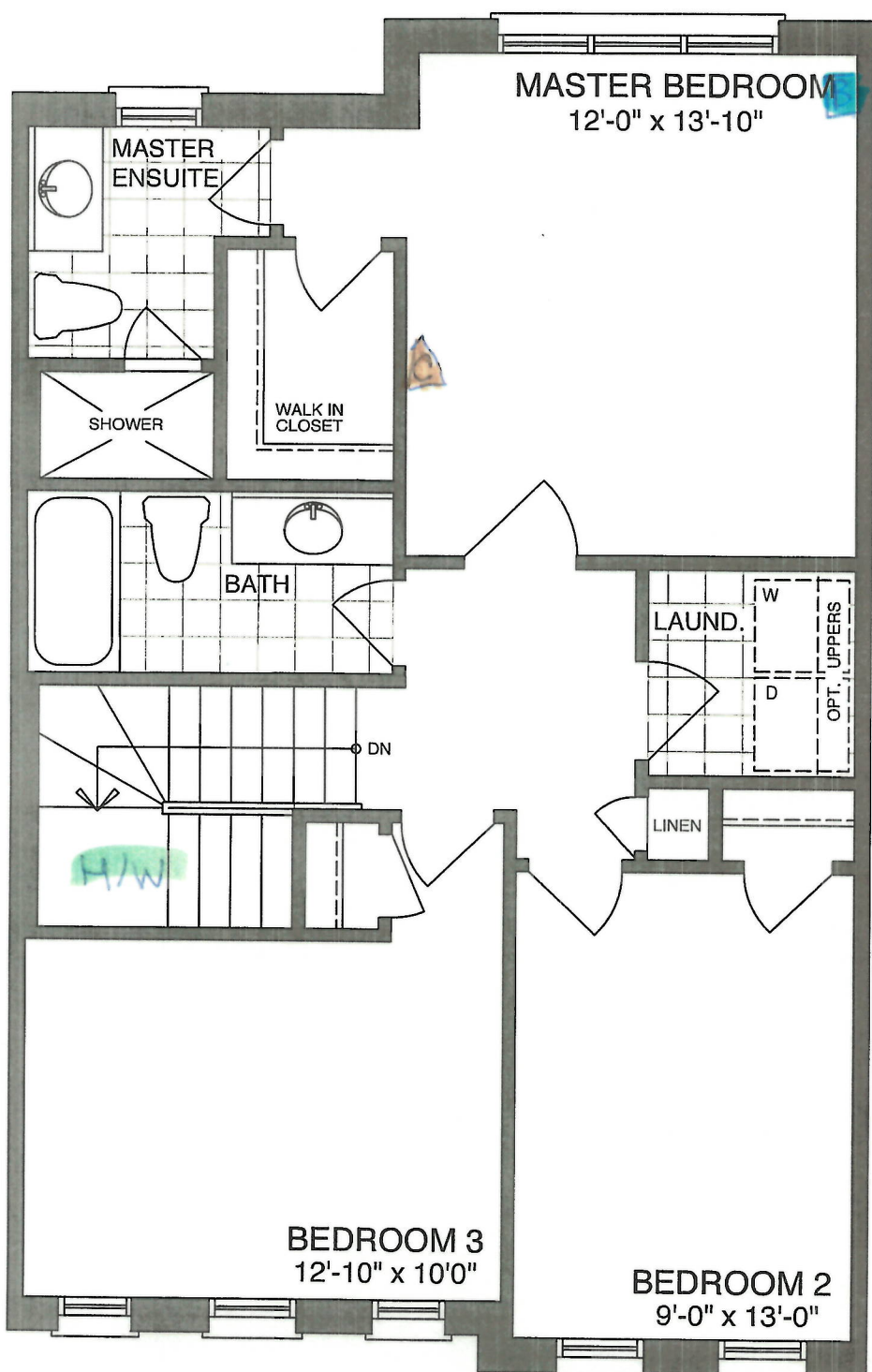
SECOND FLOOR - ELEV A1 &A2
