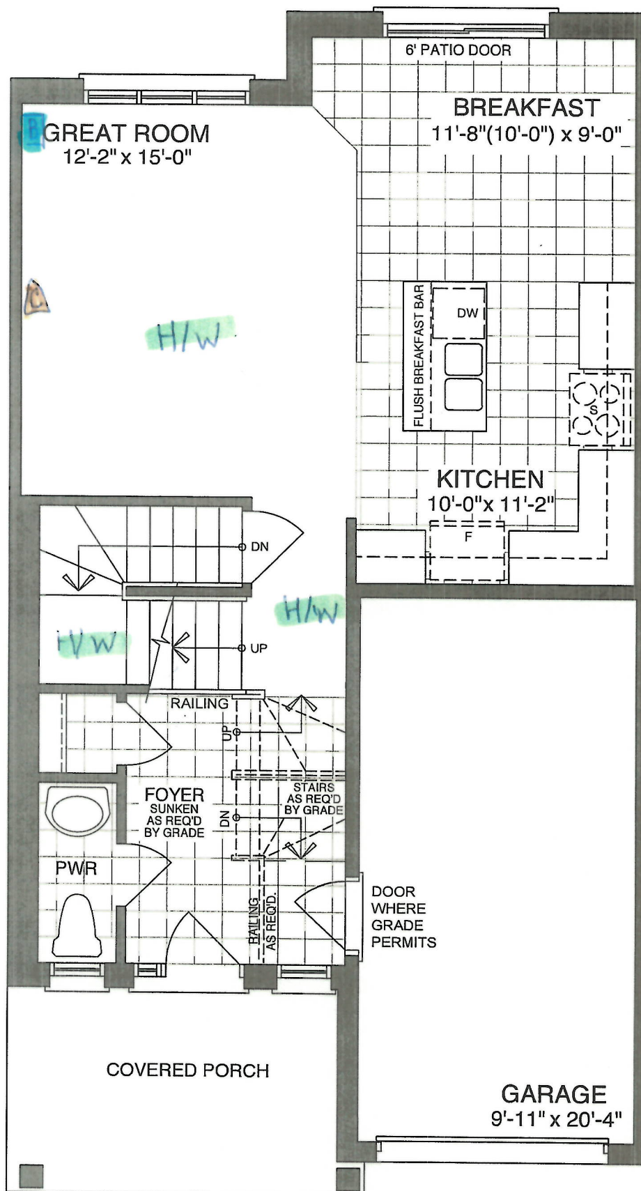
MAIN FLOOR - ELEV A & B
