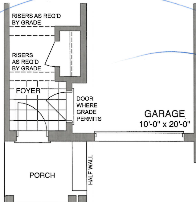
GROUND FLOOR - ELEV A3
