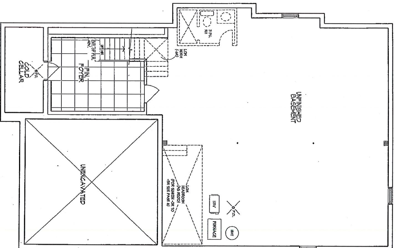
BASEMENT PLAN
