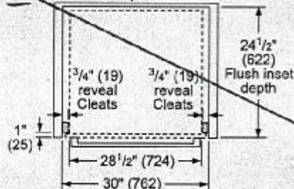
Flush installation Top view
