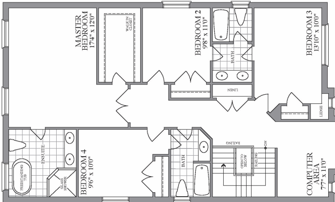
SECOND FLOOR ELEVATION A
