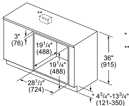
Under-counter Installation
