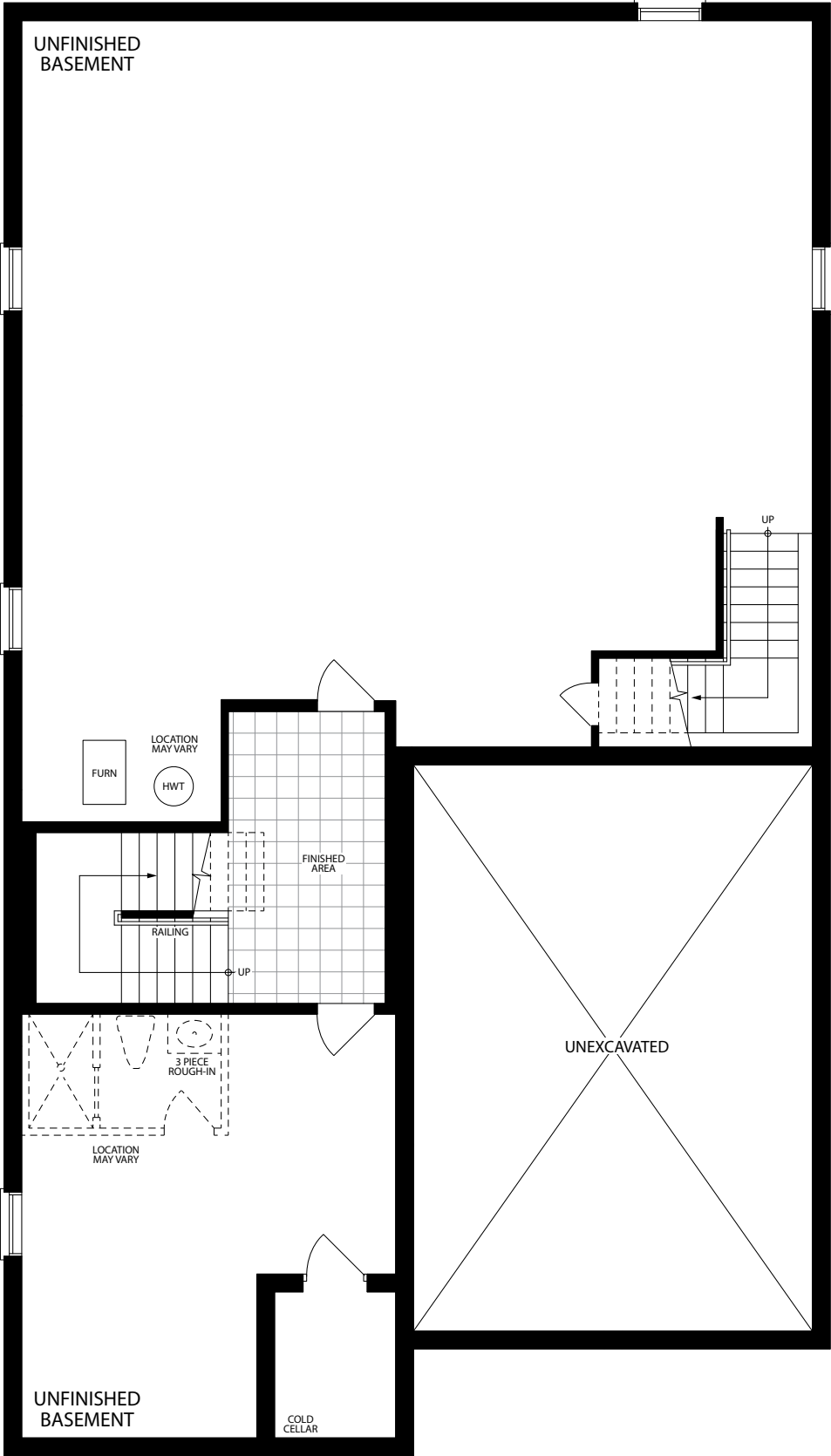
BASEMENT ELEVATION A, B & C
