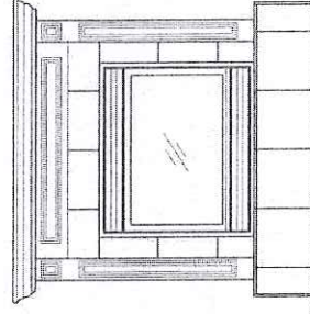
SURROUND MANTLE (PROFILE MAY VARY) AND CERAMIC SURROUND AND APPROX. 12"X12"X60" RAISED CERAMIC HEARTH (NOTE: LENGTH OF HEARTH DEPENDS ON THE MODEL OF SURROUND MANTLE)
