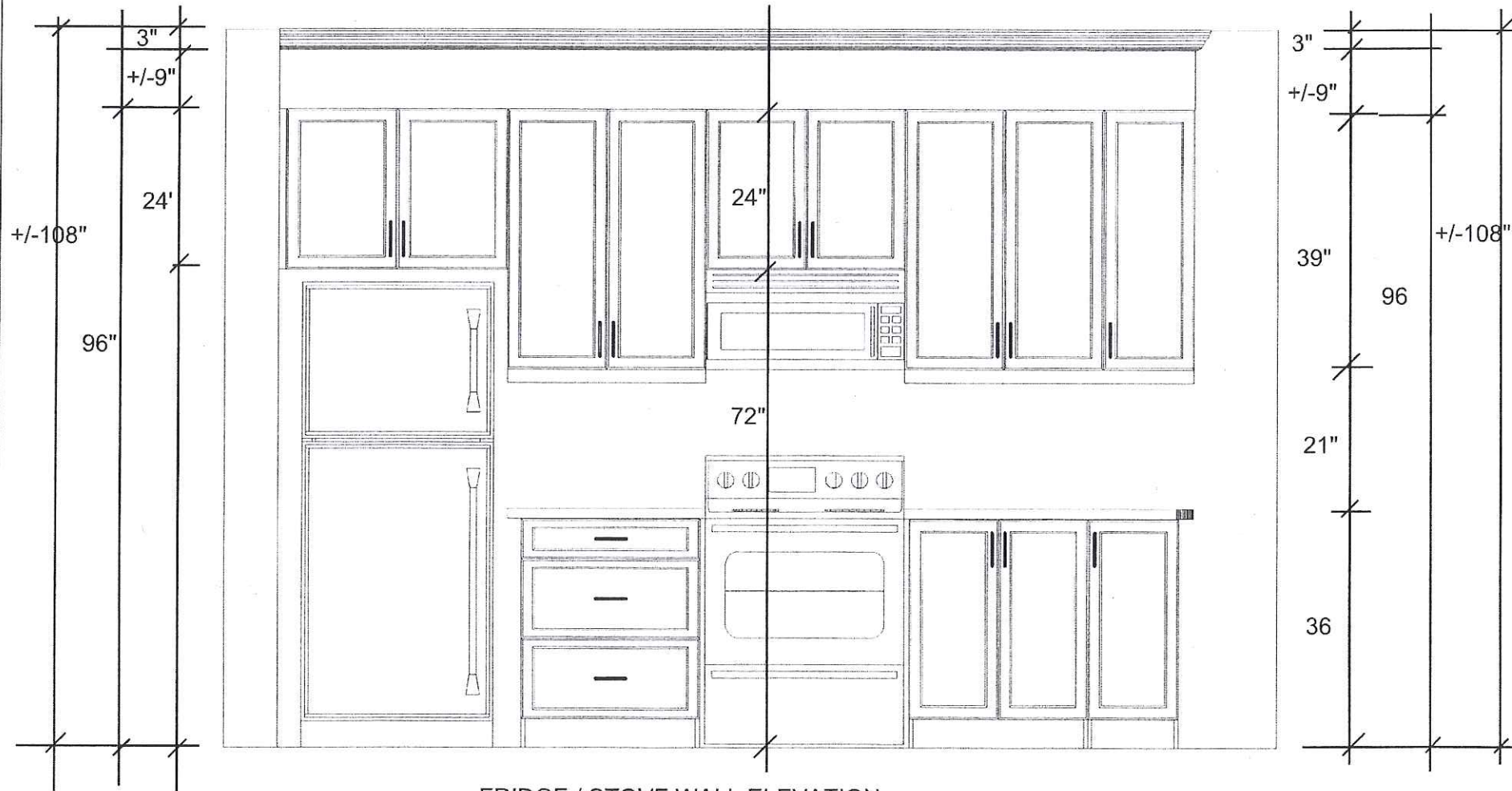
FRIDGE / STOVE WALL ELEVATION
