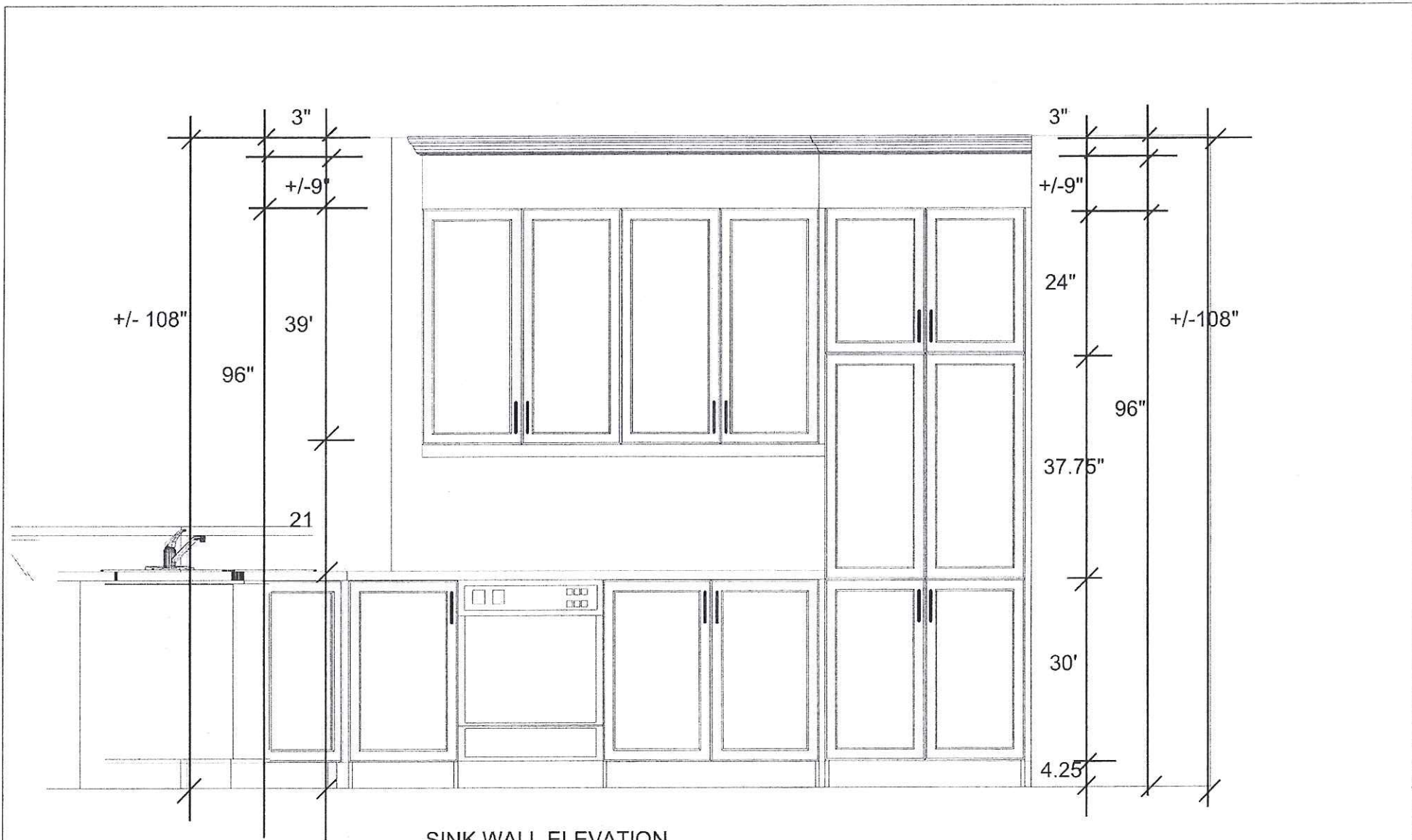
SINK WALL ELEVATION
