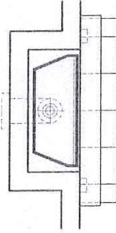
SURROUND MANTLE WITH FLAT HEARTH (NOTE: LENGTH OF HEARTH DEPENDS ON THE MODEL OF SURROUND MANTLE)
