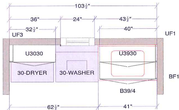
LAUNDRY ROOM
