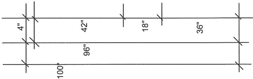
SINK WALL ELEVATION
