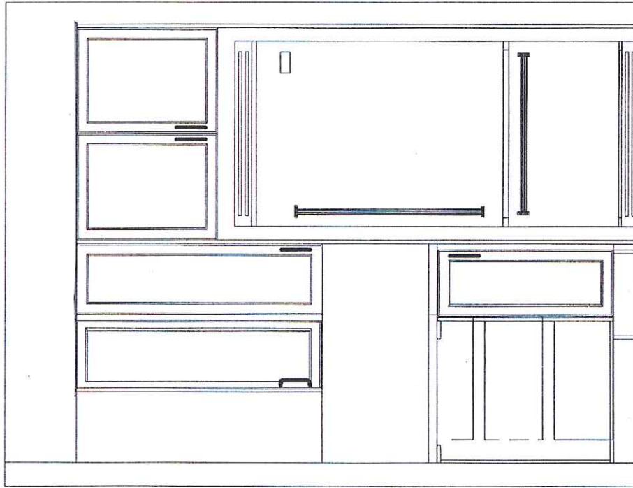
FRIDGE WALL ELEVATION
