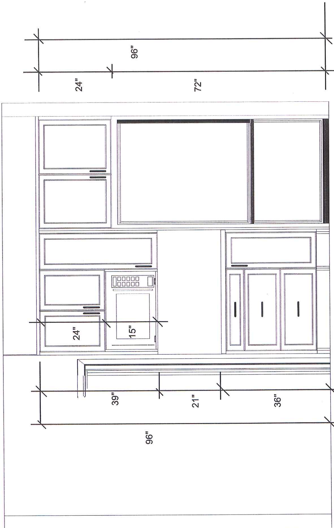
FRIDGE WALL ELEVATION
