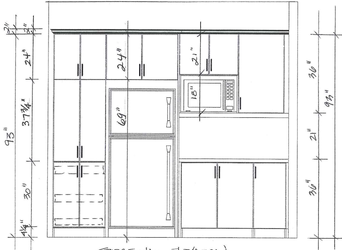
FRIDGE WALL ELEVATION
