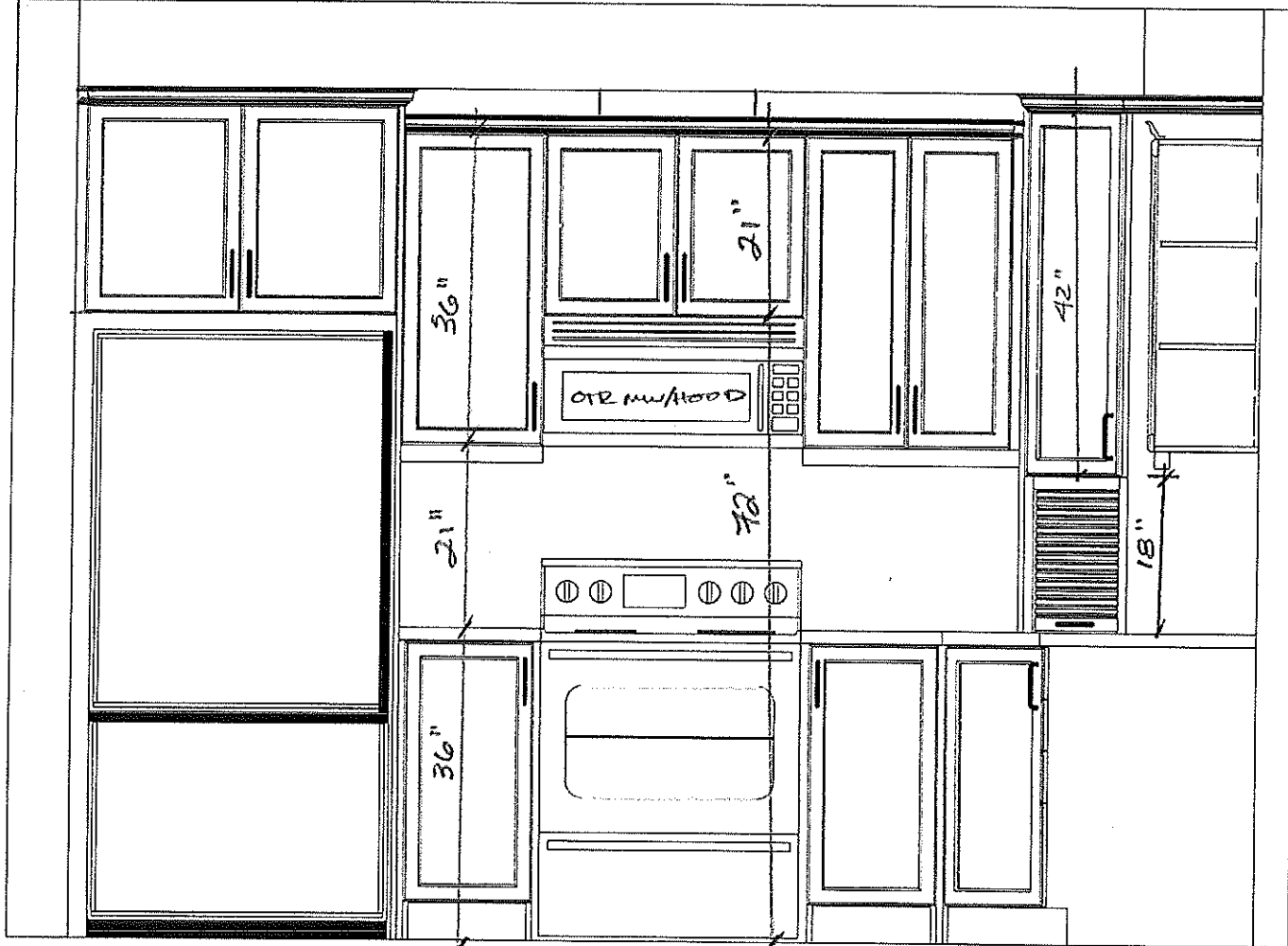
FRIDGE/STOVE WALL ELEVATION
