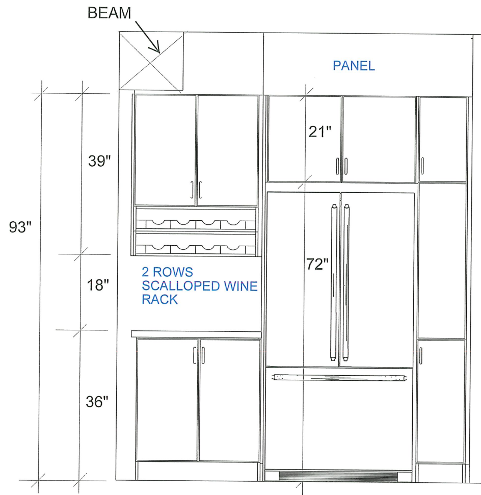
FRIDGE ELEVATION
