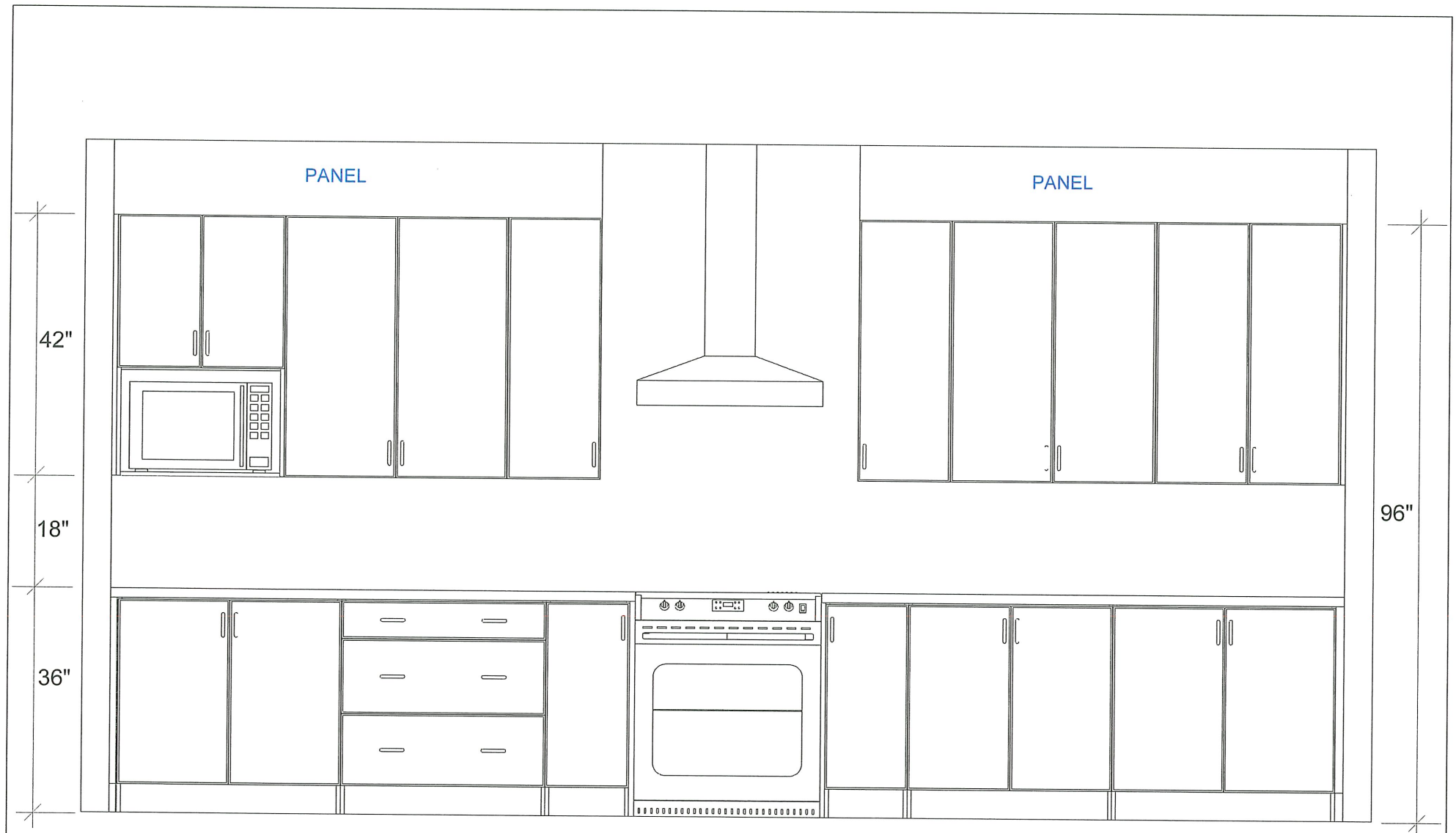
RANGE WALL ELEVATION
