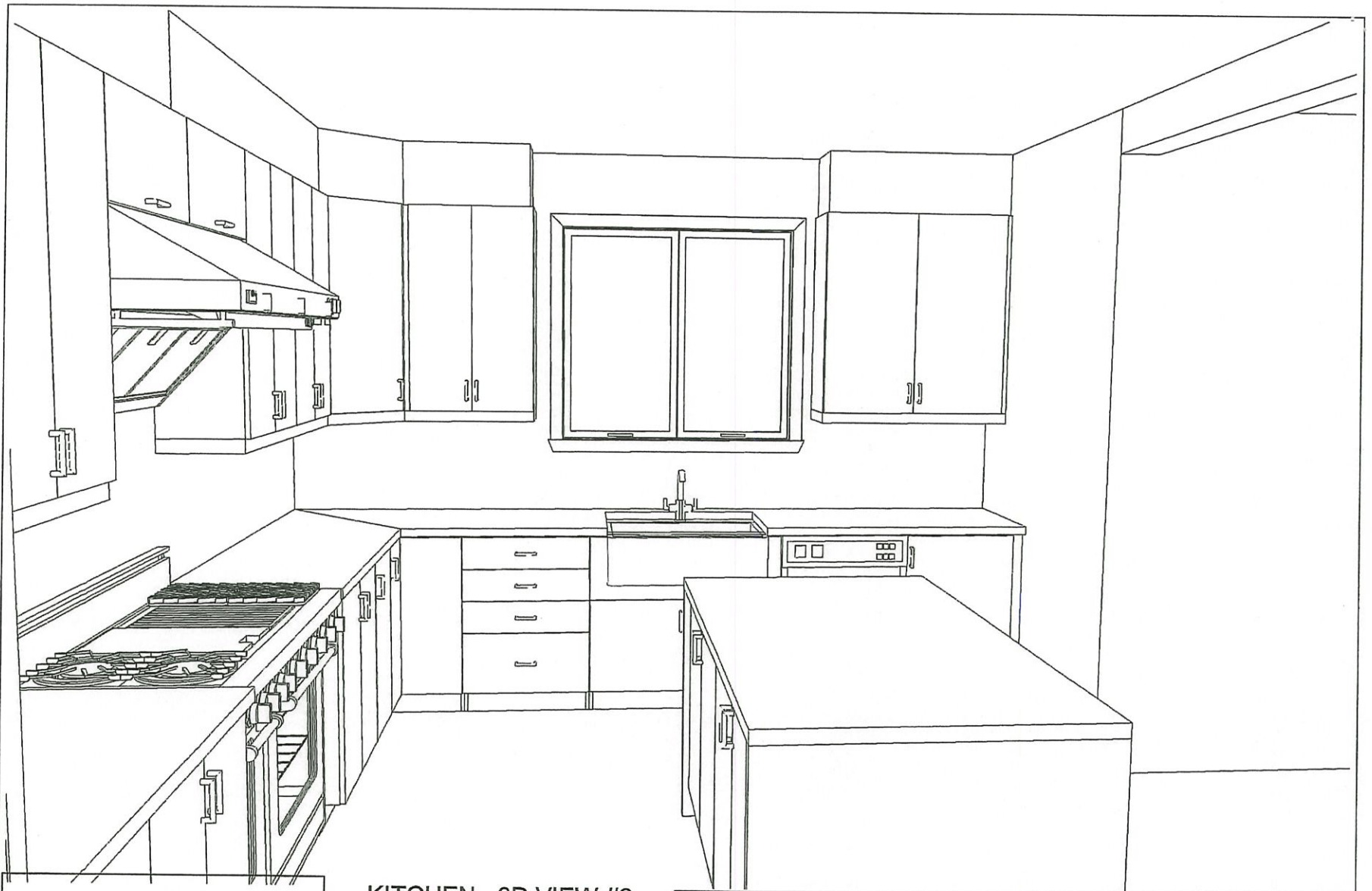
KITCHEN - 3D VIEW #2
