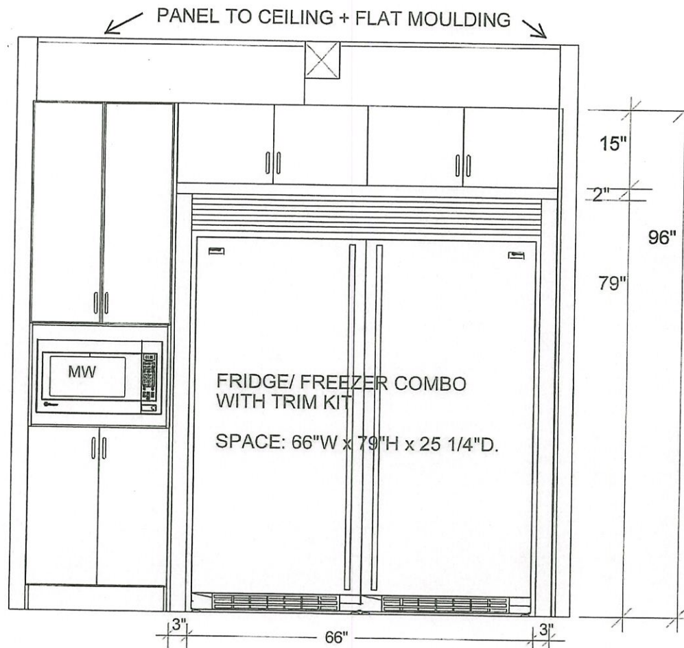
FRIDGE WALL ELEVATION
