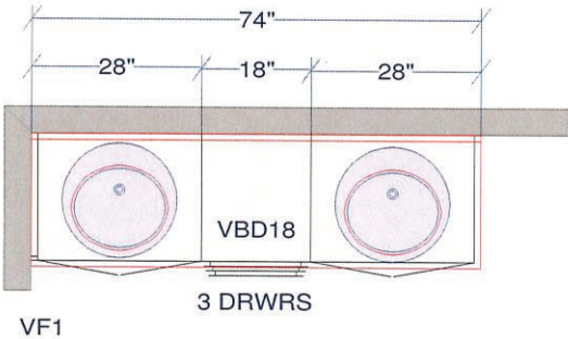
ENSUITE #2 (RE-DESIGN)
