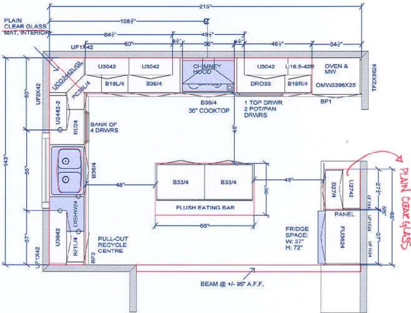
KITCHEN - FLOOR PLAN
