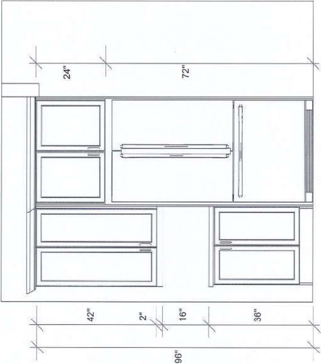
KITCHEN - FRIDGE WALL ELEVATION
