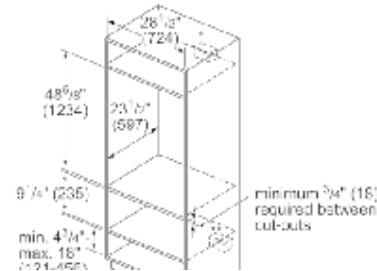
Standard Installation Combination oven over storage or warming drawer
