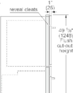
Standard Installation Combination oven over storage or warming drawer
