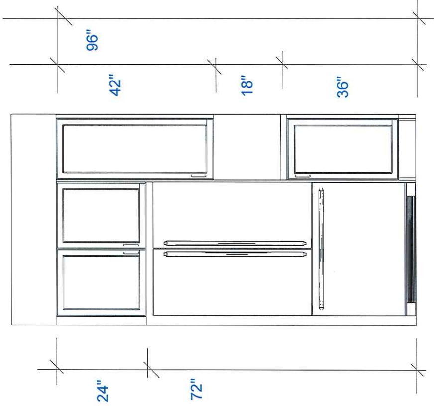
FRIDGE WALL ELEVATION
