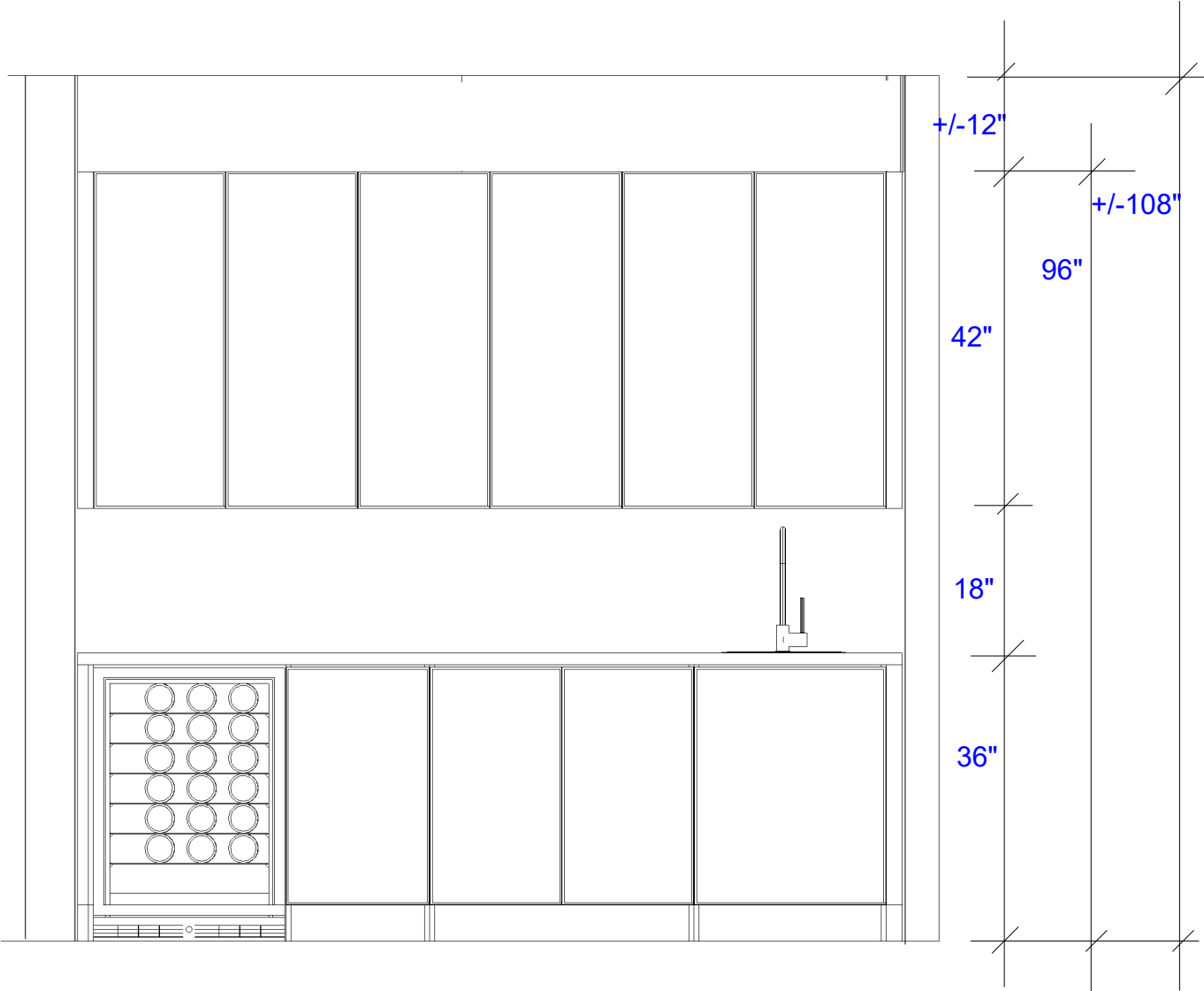
BUTLER'S PANTRY ELEVATION
