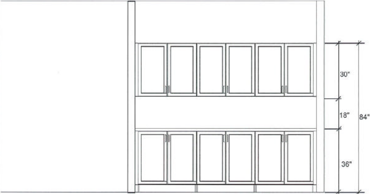
BUTLER'S PANTRY WALL ELEVATION NEWINGTON III - CHEF'S KITCHEN
