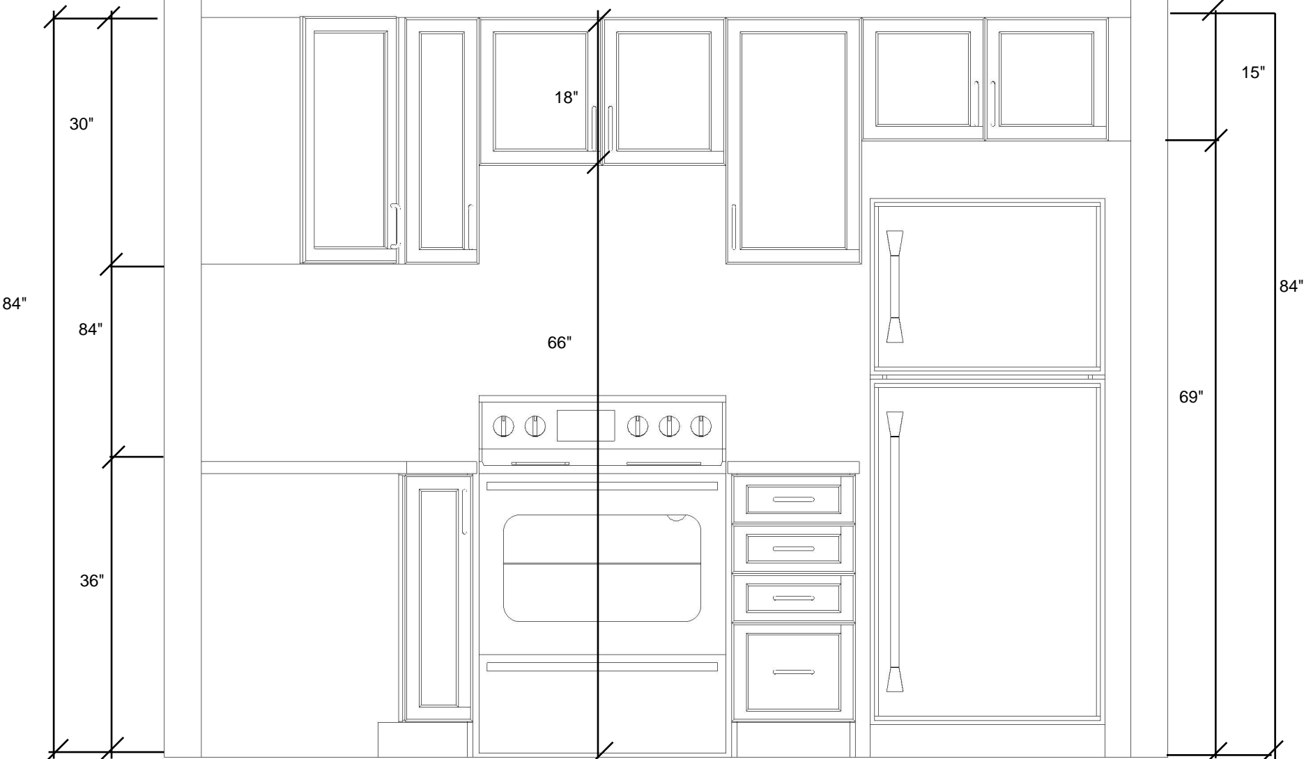
BASEMENT KITCHEN - RANGE / FRIDGE WALL ELEVATION 35- 32 MIRAPOSA
