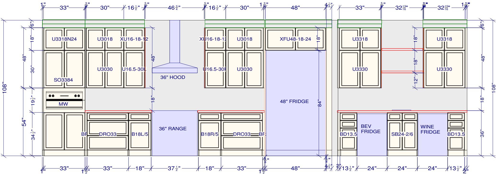
RANGE / FRIDGE WALL ELEVATION
