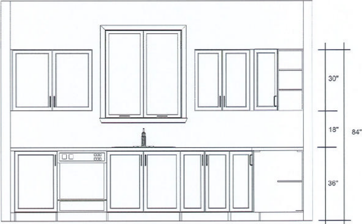
SINK WALL ELEVATION 509 ANNAPOLIS
