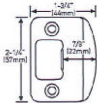
FULL LIP RADIUS STRIKE
