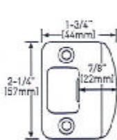
FULL LIP RADIUS STRIKE
