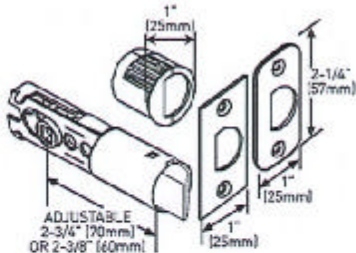
6-IN-1 PRIVACY/PASSAGE LATCH
