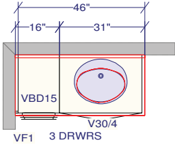
IN LAW - ENSUITE
