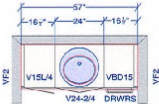
BSMT APT VANITY
